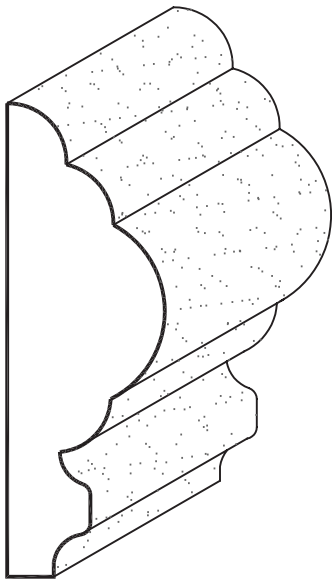
GH 406 ( \frac{3}{4} " X 2 \frac{7}{16} " )
