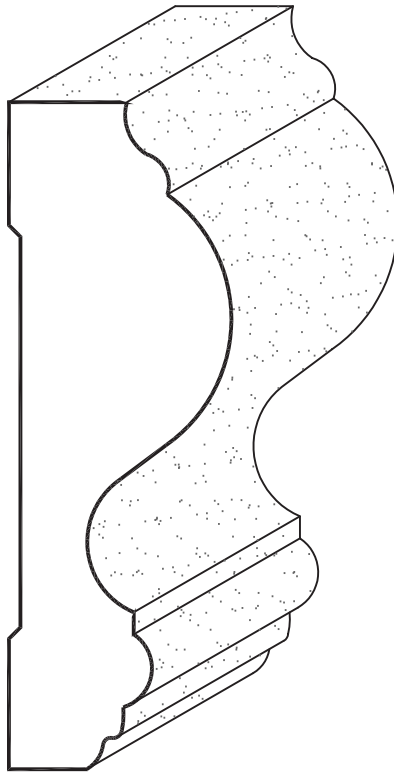
GH 413 ( 1\frac{1}{8} " X 3\frac{1}{2} ")
