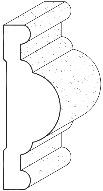
GH 411 ( 1\frac{1}{8} " X 3\frac{1}{2} " )
